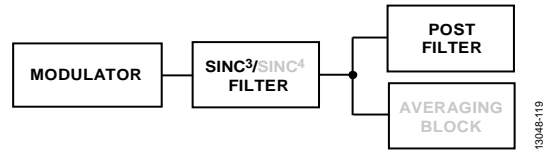
Figure 112. Post Filters
