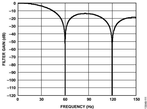
Figure 104. 60 Hz Rejection
