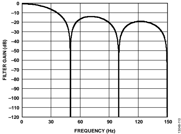
Figure 103. 50 Hz Rejection
