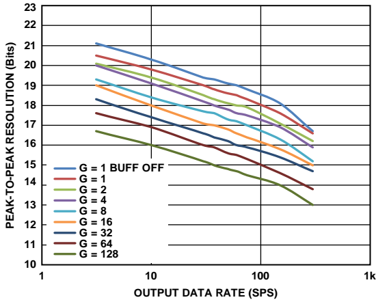
Figure 58. Peak-to-Peak Resolution vs. Output Data Rate, Sinc^4 + Sinc^1 Filter (Low Power Mode)
